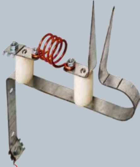
Lightning diverter Install at top of the pipe
